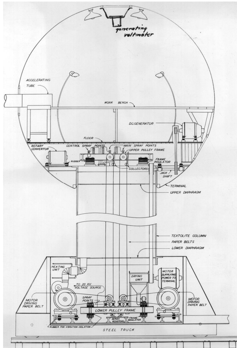
DIAGRAM OF THE MACHINE AS ORIGINALLY SET UP AT ROUND HILL NOTICE THAT THE ORIGINAL CHARGING BELTS WERE PAPER!
